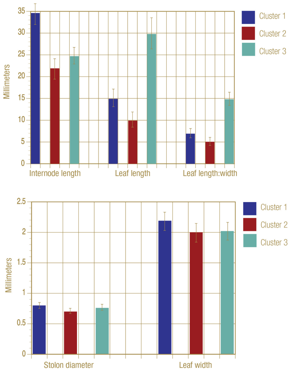
Figure 2. Cluster means and standard deviations for internode length, leaf length, leaf length:width ratio, stolon diameter and leaf width measurements. Measurements were made on 52 off-type and desirable ultradwarf bermudagrass samples harvested from golf course putting greens in the southeastern U.S.
